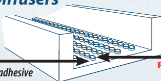
Diffusers
