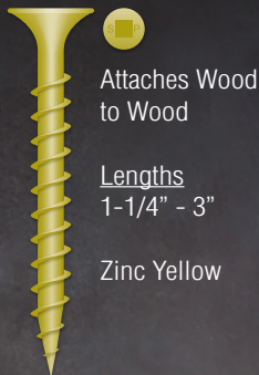
Square Drive Bugle Head Coarse Thread
