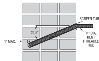
Configuration B (Tension & Shear)
